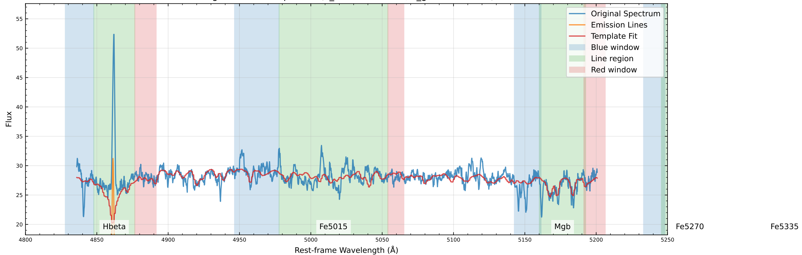
Original Data Comparison (v_star=20.7 km/s, v_gas=29.3 km/s)
