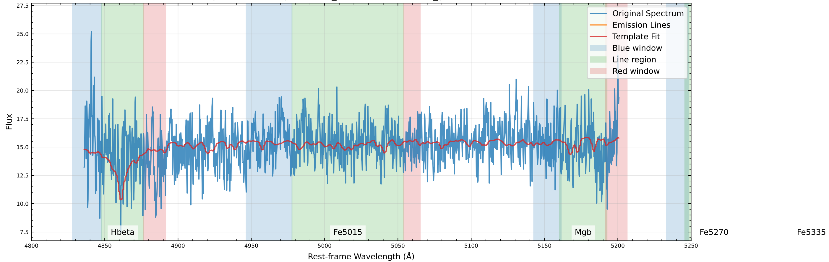
Original Data Comparison (v_star=1039.4 km/s, v_gas=1278.8 km/s)
