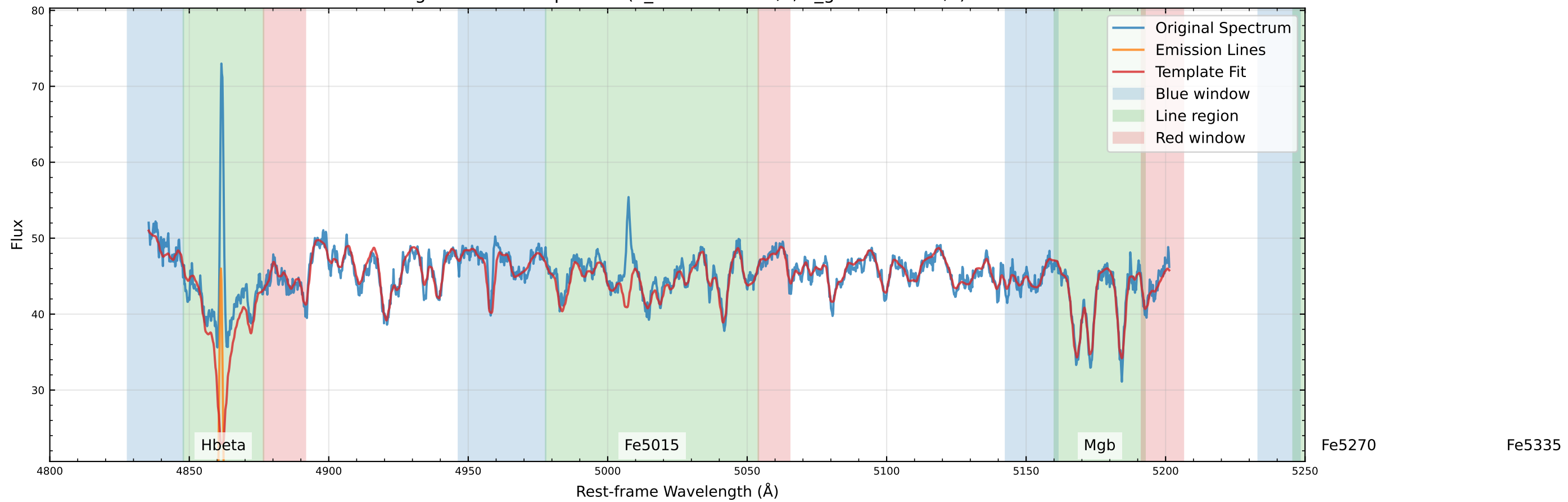
Original Data Comparison (v_star=31.4 km/s, v_gas=22.8 km/s)
