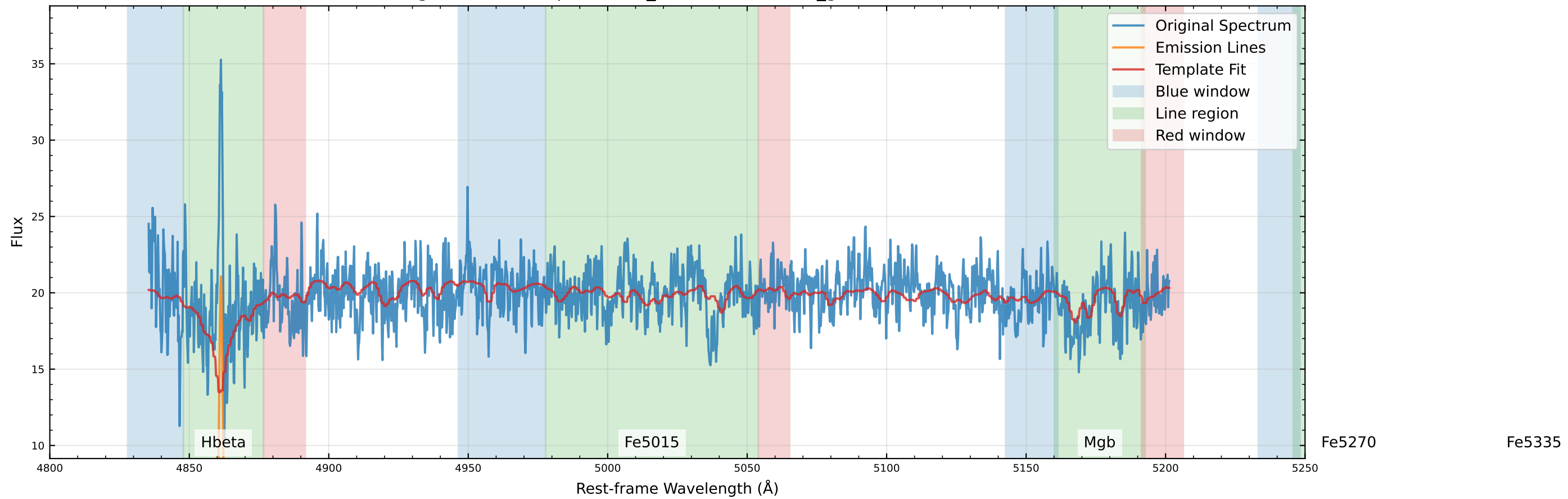
Original Data Comparison (v_star=10.8 km/s, v_gas=-5.8 km/s)
