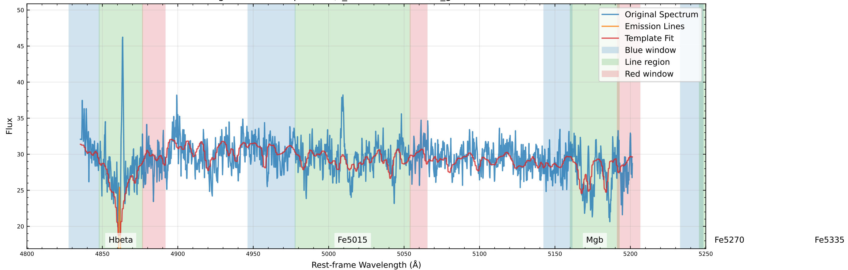
Original Data Comparison (v_star=116.4 km/s, v_gas=125.0 km/s)
