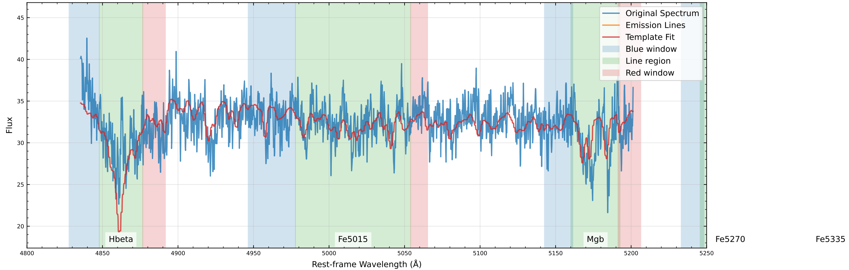
Original Data Comparison ( v_{\text{star}}=92.3 km/s, v_{\text{gas}}=100.1 km/s)
