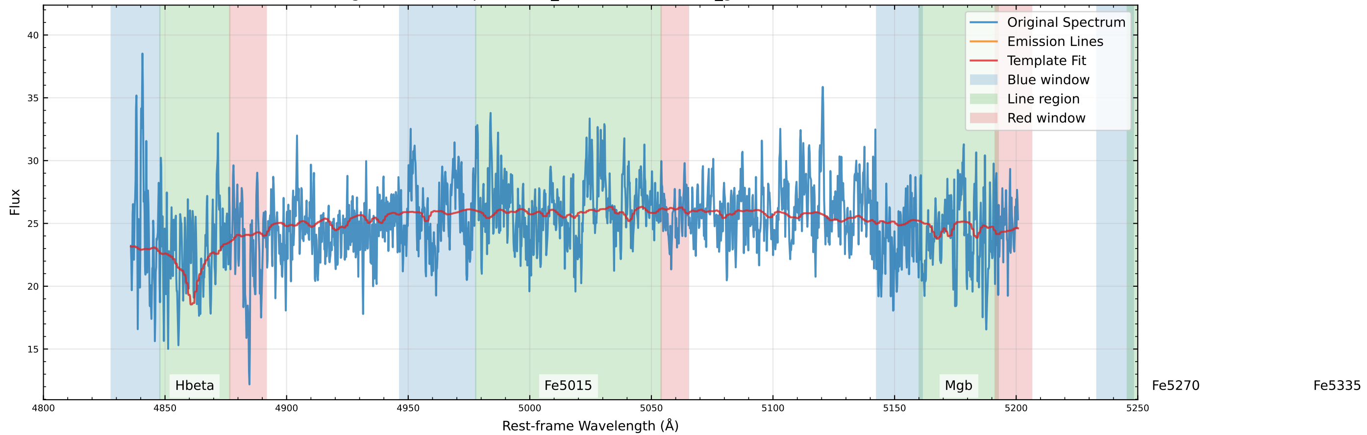
Original Data Comparison (v_star=-136.2 km/s, v_gas=-75.3 km/s)
