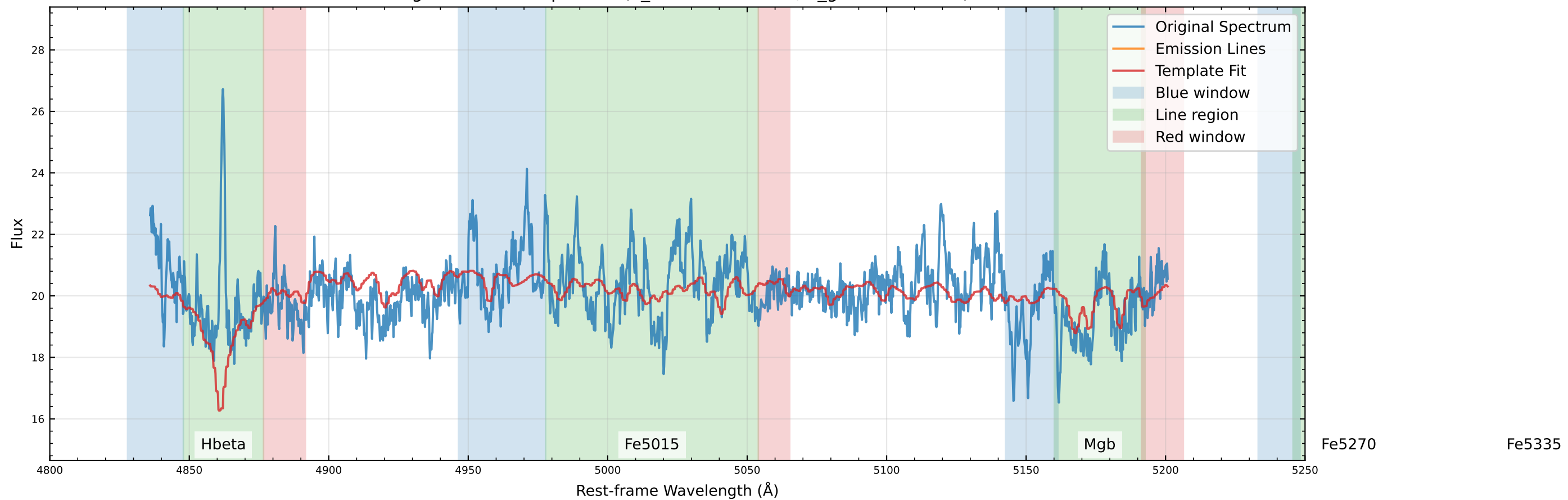
Original Data Comparison (v_star=-19.4 km/s, v_gas=36.6 km/s)
