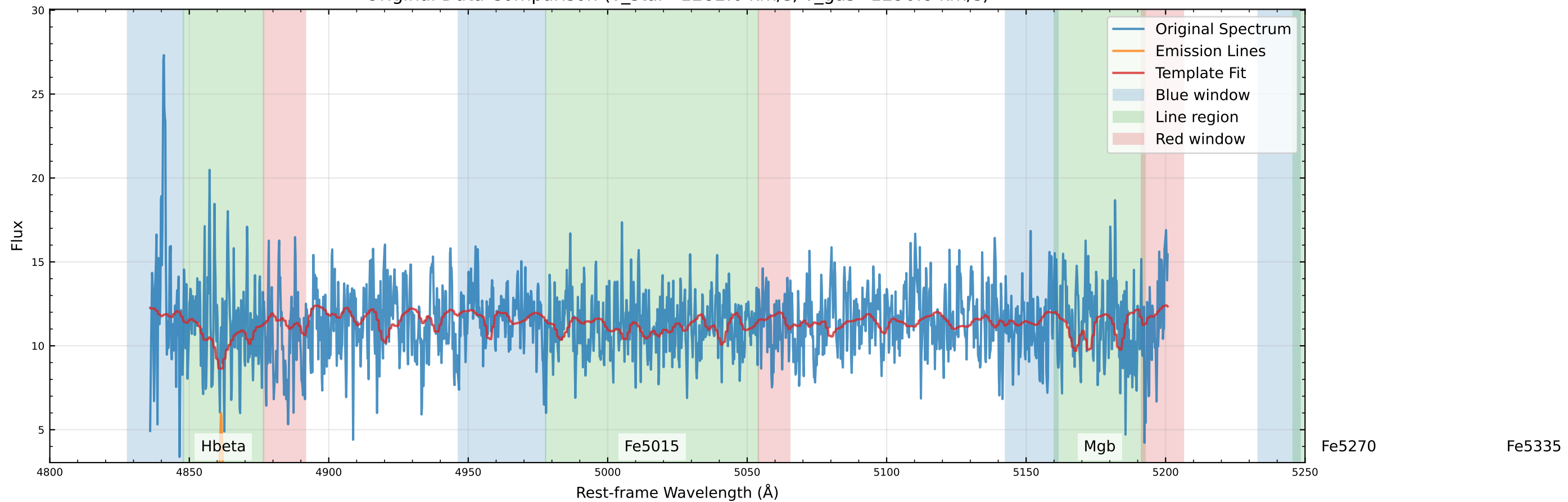
Original Data Comparison (v_star=1282.6 km/s, v_gas=1290.8 km/s)
