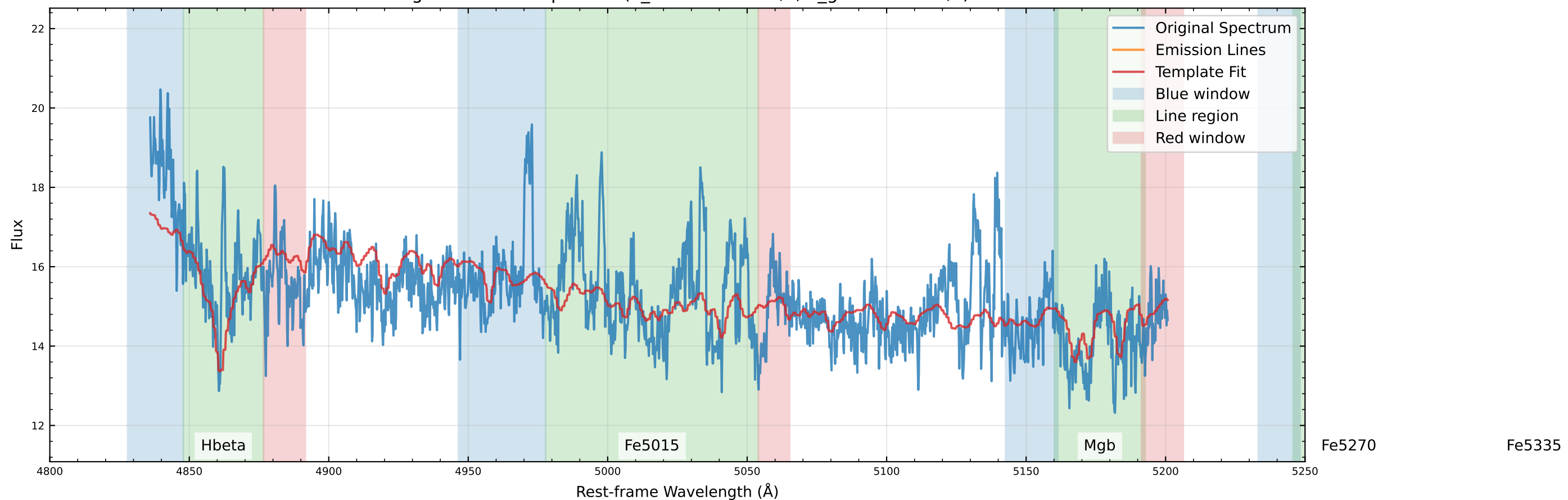
Original Data Comparison (v_star=-32.3 km/s, v_gas=62.5 km/s)
