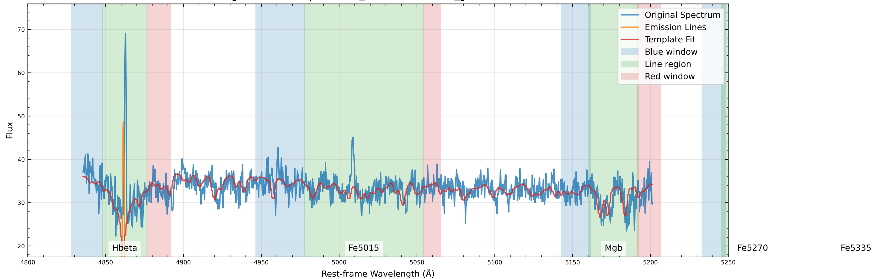
Original Data Comparison (v_star=93.5 km/s, v_gas=82.7 km/s)
