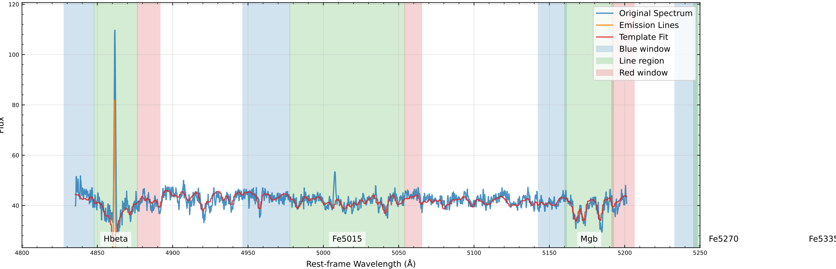
Original Data Comparison (v_star=35.9 km/s, v_gas=20.9 km/s)
