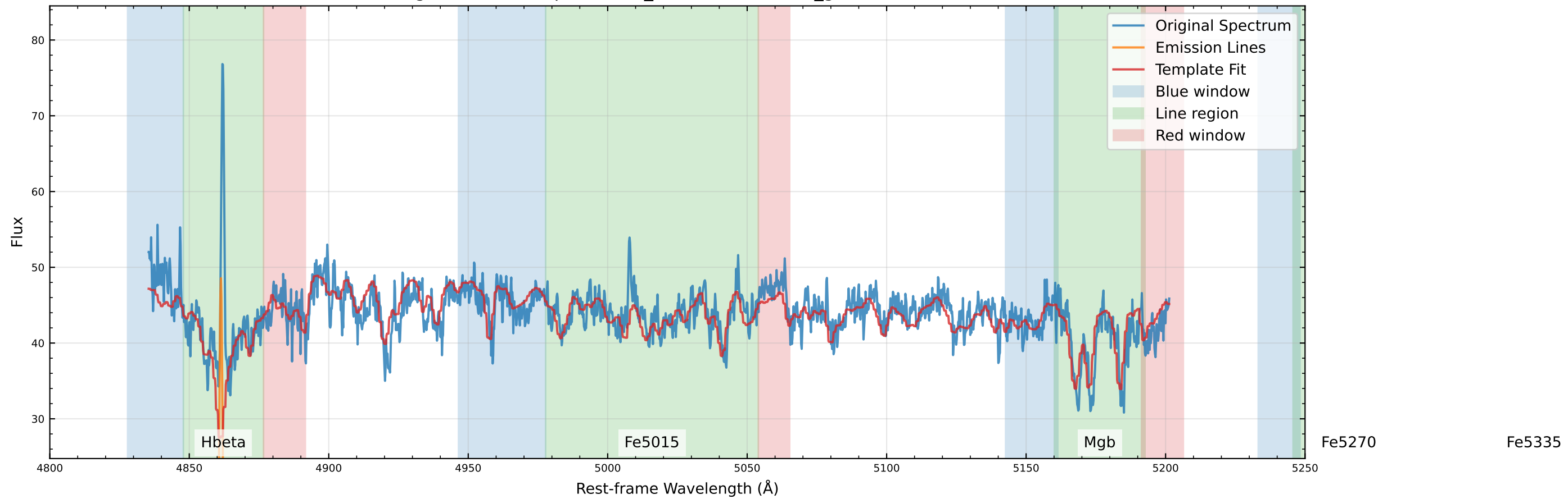
Original Data Comparison (v_star=49.7 km/s, v_gas=41.0 km/s)
