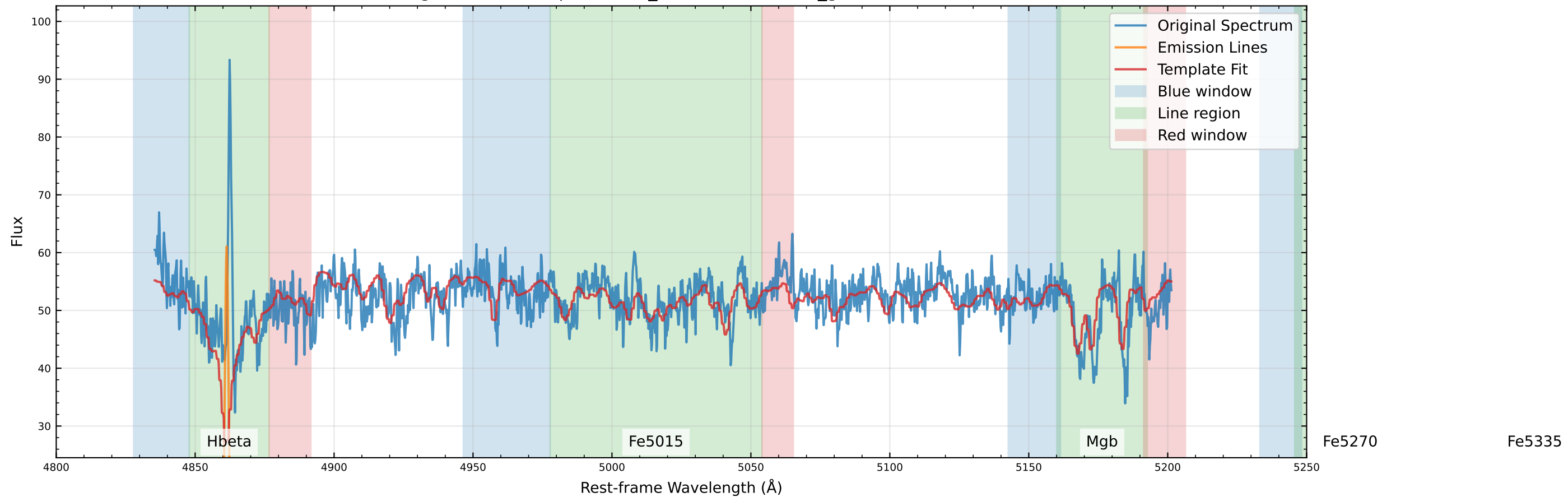
Original Data Comparison (v_star=77.4 km/s, v_gas=71.5 km/s)
