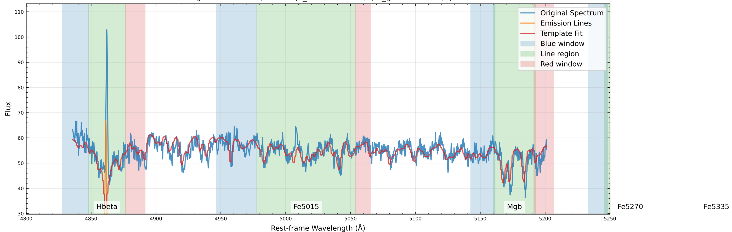
Original Data Comparison (v_star=67.9 km/s, v_gas=48.8 km/s)
