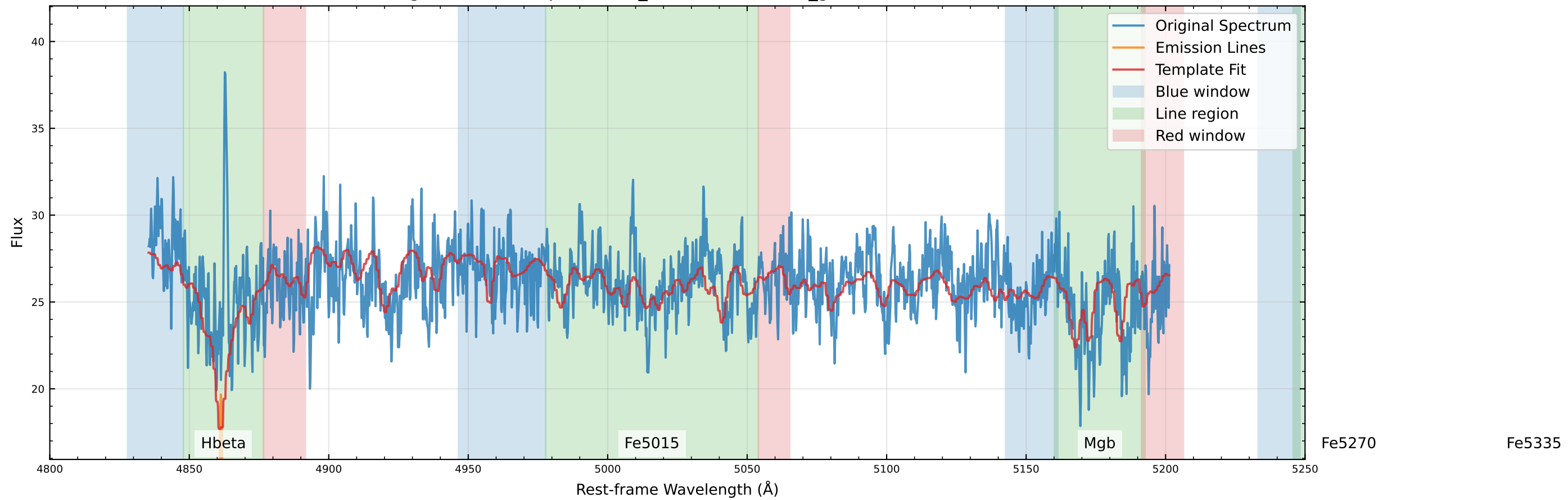
Original Data Comparison ( v_{\text{star}}=96.7 km/s, v_{\text{gas}}=103.4 km/s)
