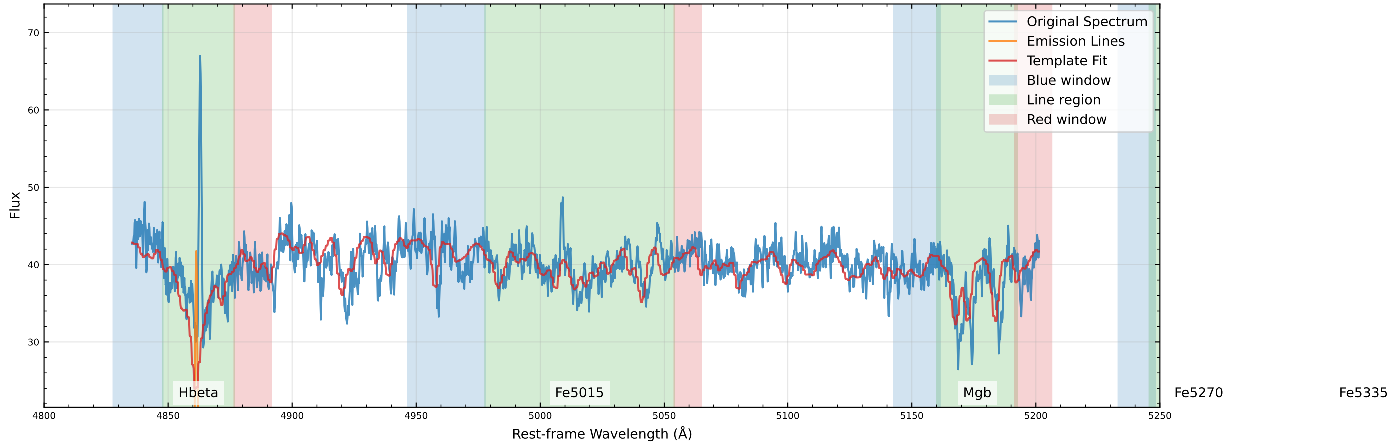
Original Data Comparison (v_star=96.5 km/s, v_gas=99.9 km/s)
