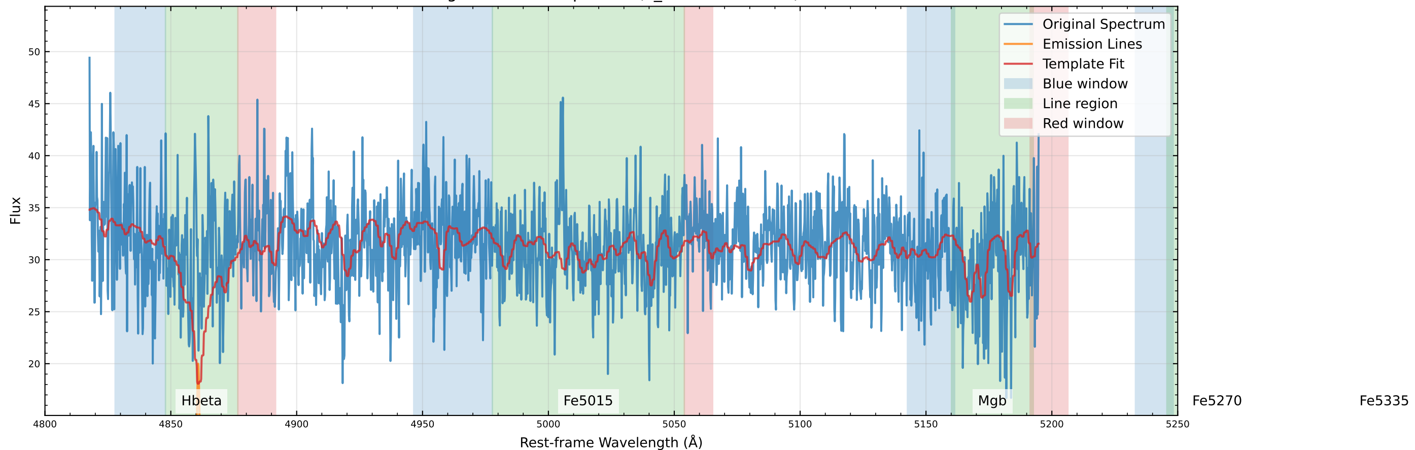
Original Data Comparison (v_star=-68.6 km/s)
