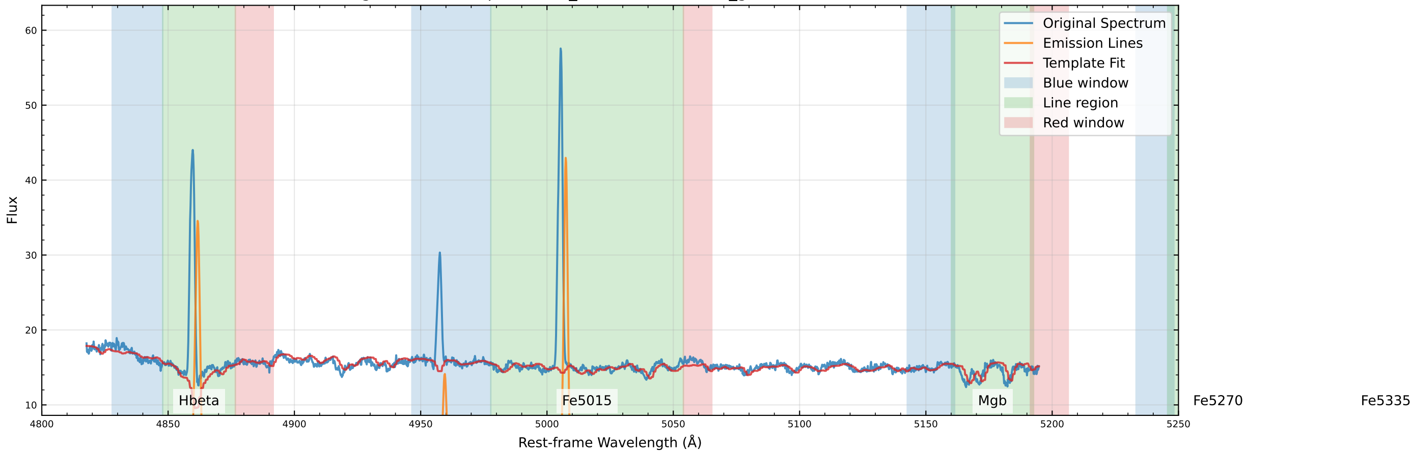
Original Data Comparison (v_star=-90.1 km/s, v_gas=-126.6 km/s)
