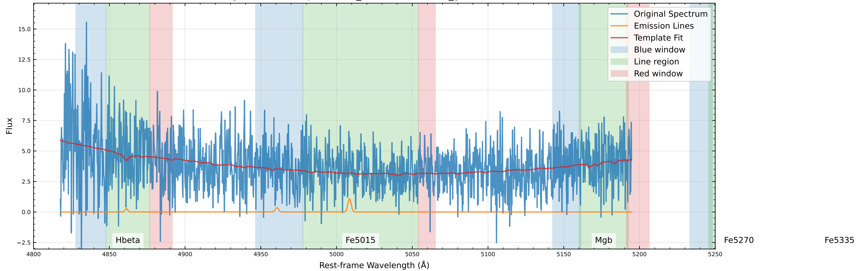
Original Data Comparison (v_star=27.4 km/s, v_gas=25.0 km/s)
