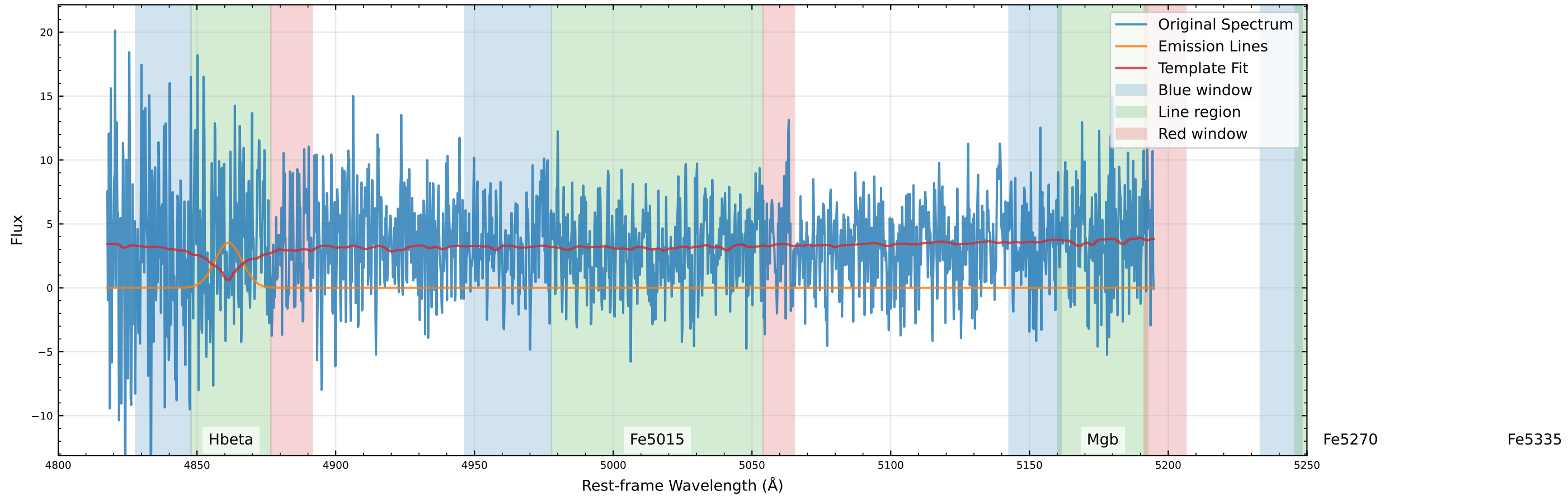
Original Data Comparison (v_star=89.8 km/s, v_gas=308.6 km/s)
