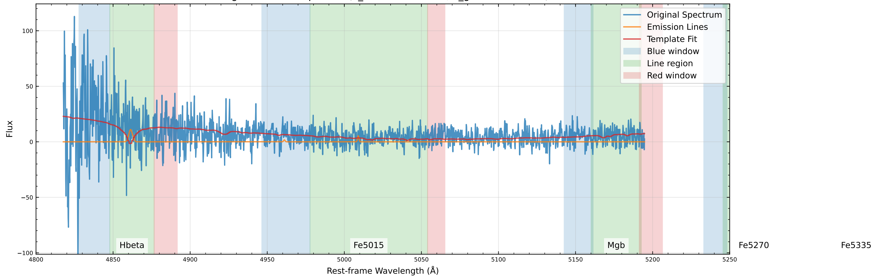
Original Data Comparison (v_star=799.7 km/s, v_gas=596.0 km/s)
