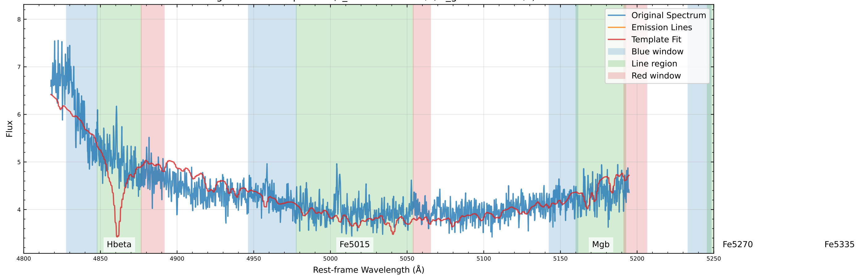
Original Data Comparison (v_star=-153.5 km/s, v_gas=139.3 km/s)
