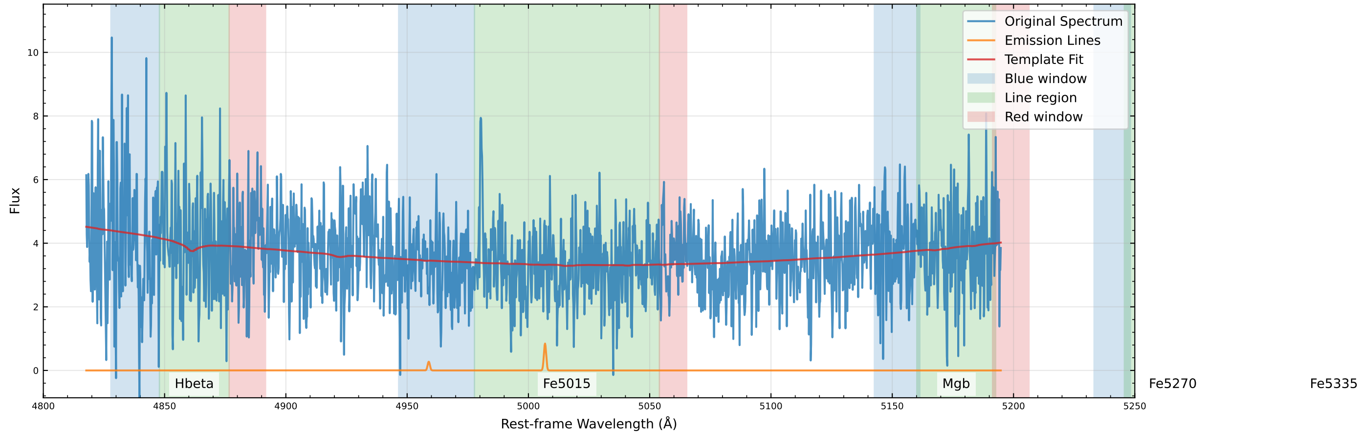
Original Data Comparison (v_star=-242.7 km/s, v_gas=-278.6 km/s)
