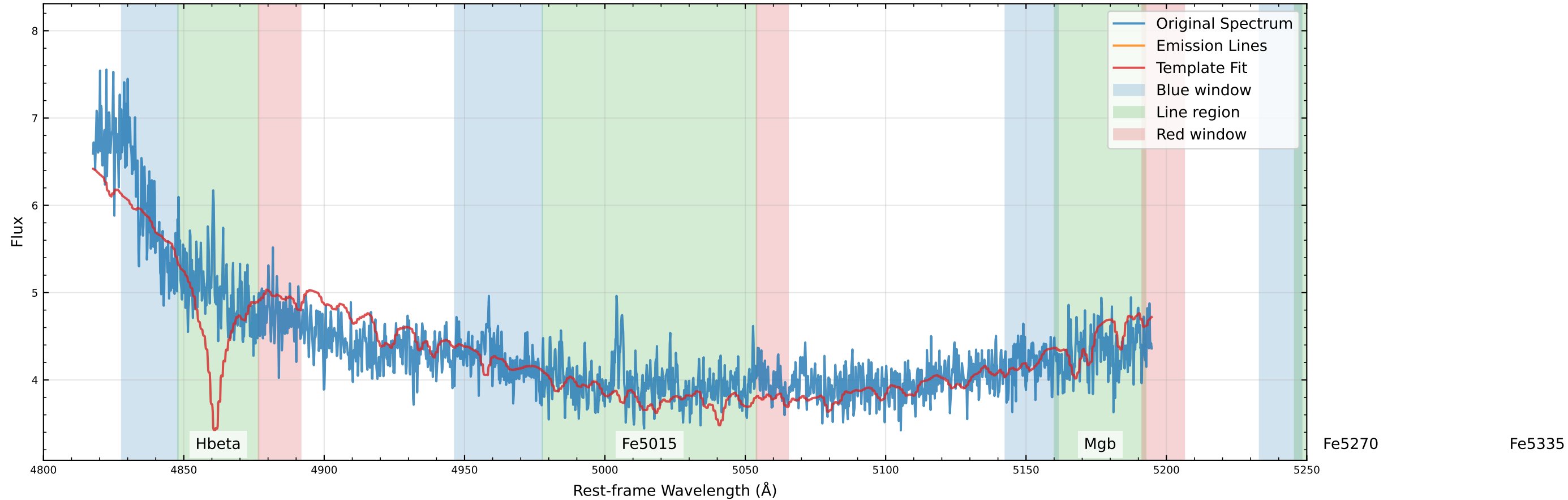
Original Data Comparison (v_star=-153.5 km/s, v_gas=139.3 km/s)
