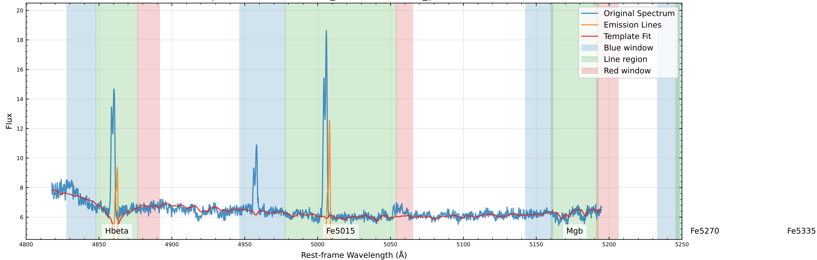
Original Data Comparison (v_star=-97.5 km/s, v_gas=-131.7 km/s)
