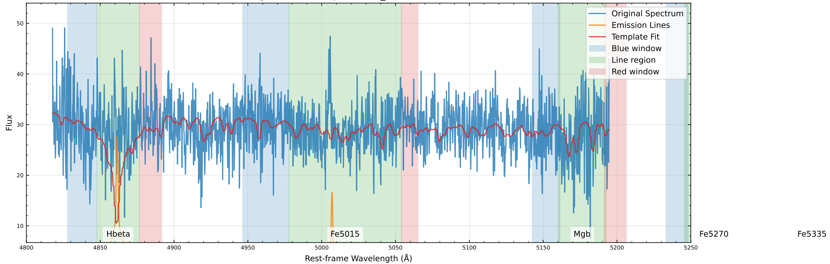
Original Data Comparison (v_star=-101.6 km/s)
