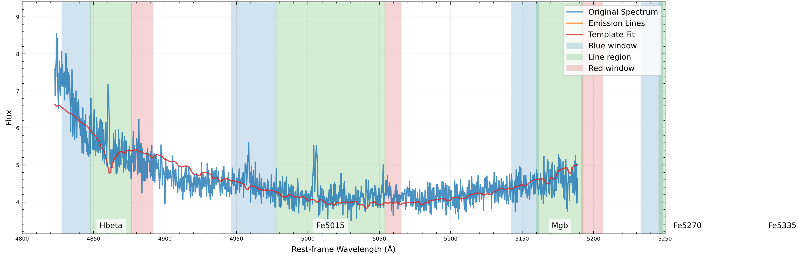
Original Data Comparison (v_star=-299.8 km/s, v_gas=-71.0 km/s)
