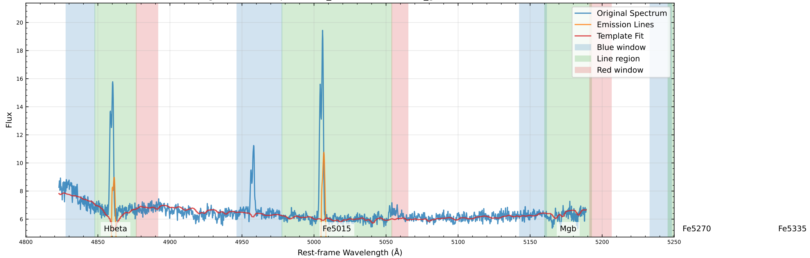
Original Data Comparison (v_star=-117.6 km/s, v_gas=-78.6 km/s)
