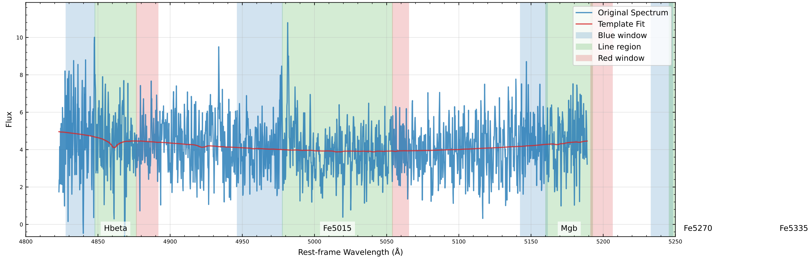
Original Data Comparison (v_star=-58.3 km/s)
