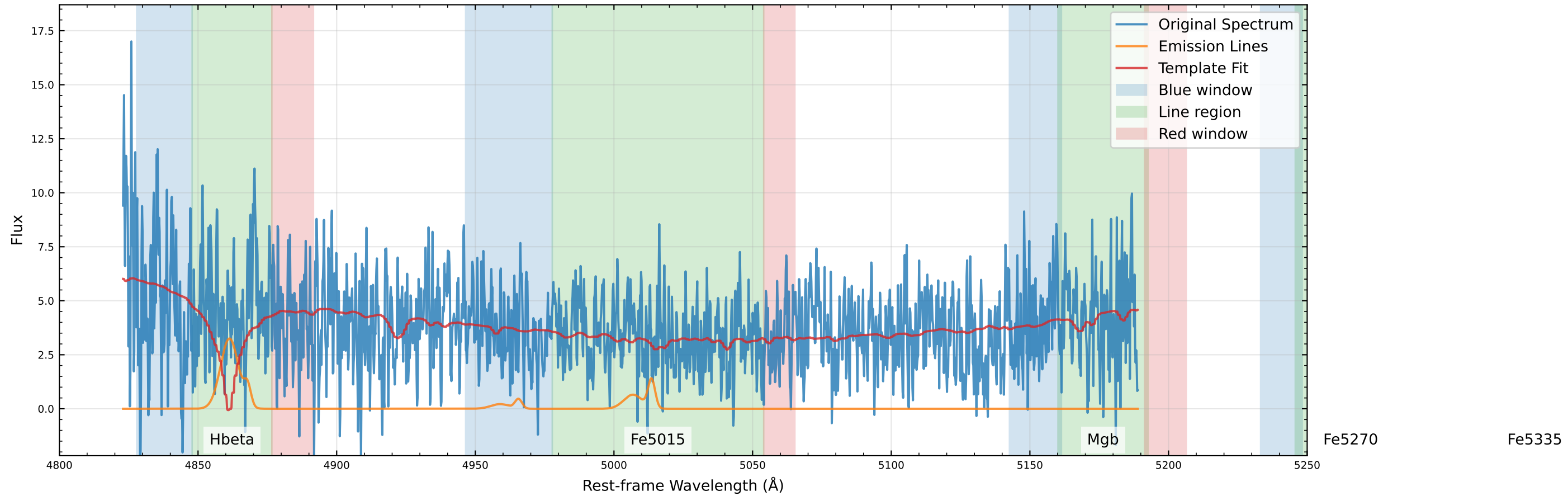
Original Data Comparison (v_star=-137.8 km/s, v_gas=-437.8 km/s)
