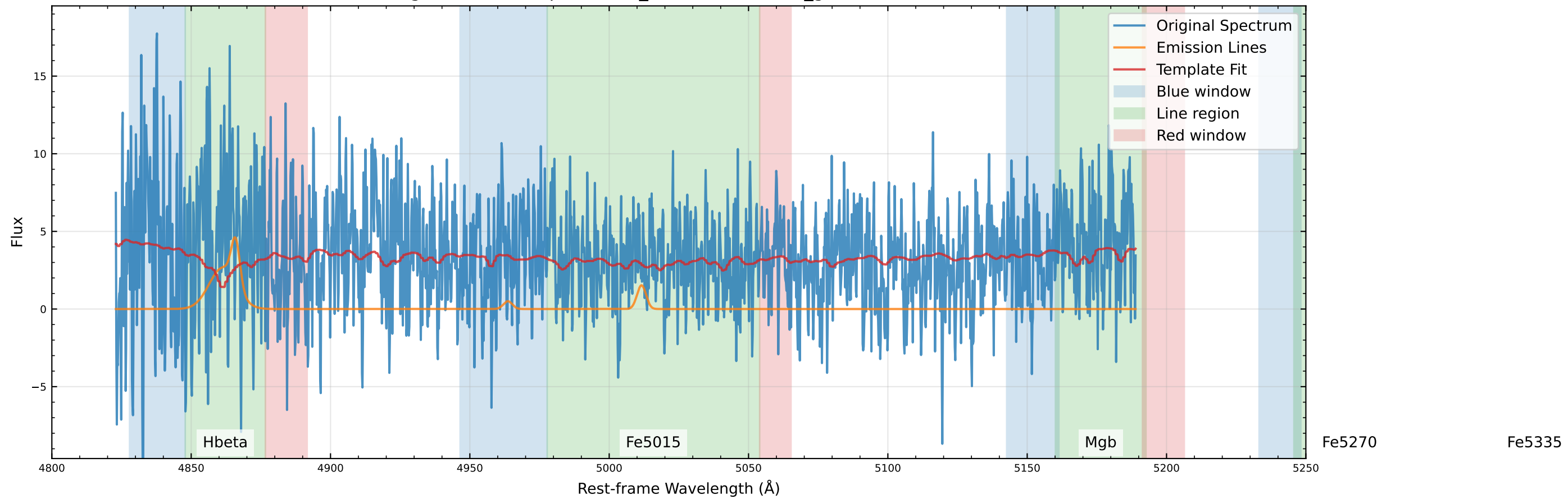
Original Data Comparison (v_star=-8.1 km/s, v_gas=-112.5 km/s)
