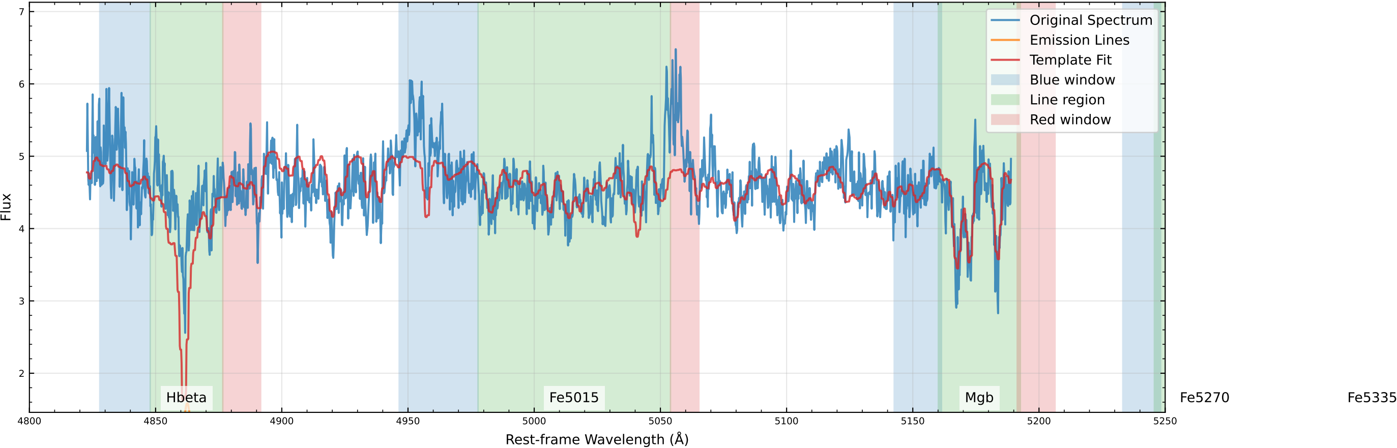
Original Data Comparison (v_star=-9.3 km/s, v_gas=-84.9 km/s)
