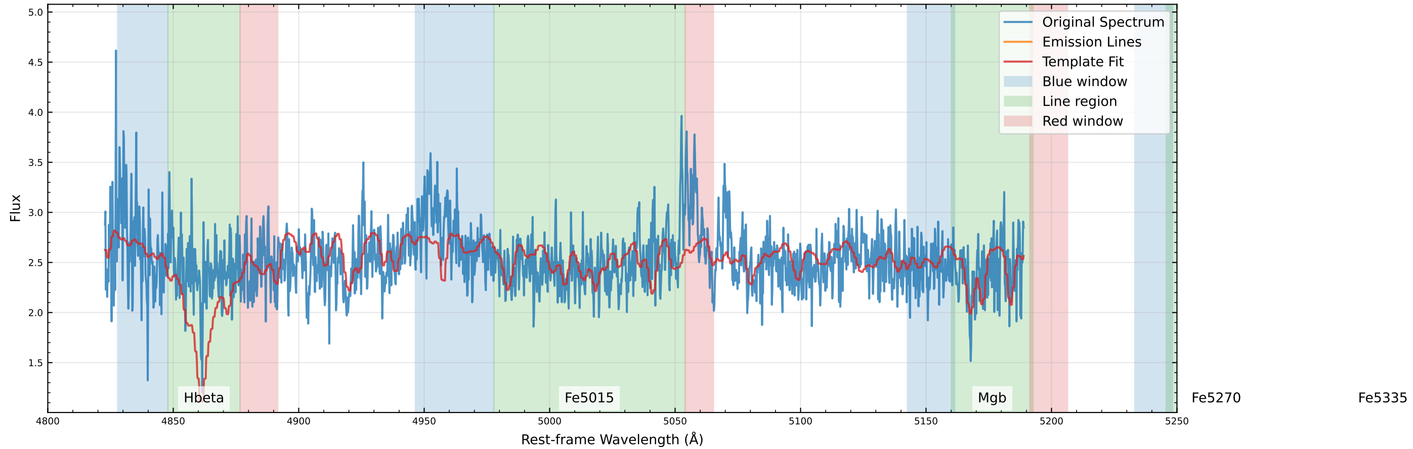
Original Data Comparison (v_star=-83.7 km/s, v_gas=-255.1 km/s)
