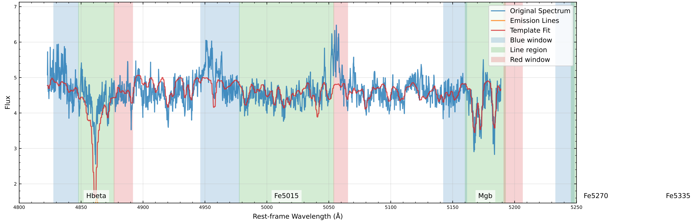
Original Data Comparison (v_star=-9.3 km/s, v_gas=-84.9 km/s)
