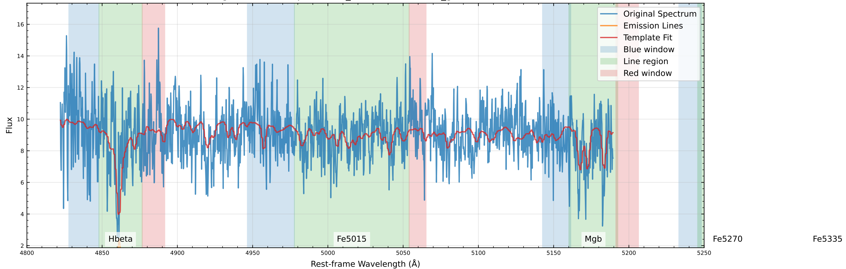
Original Data Comparison (v_star=-19.0 km/s, v_gas=60.7 km/s)
