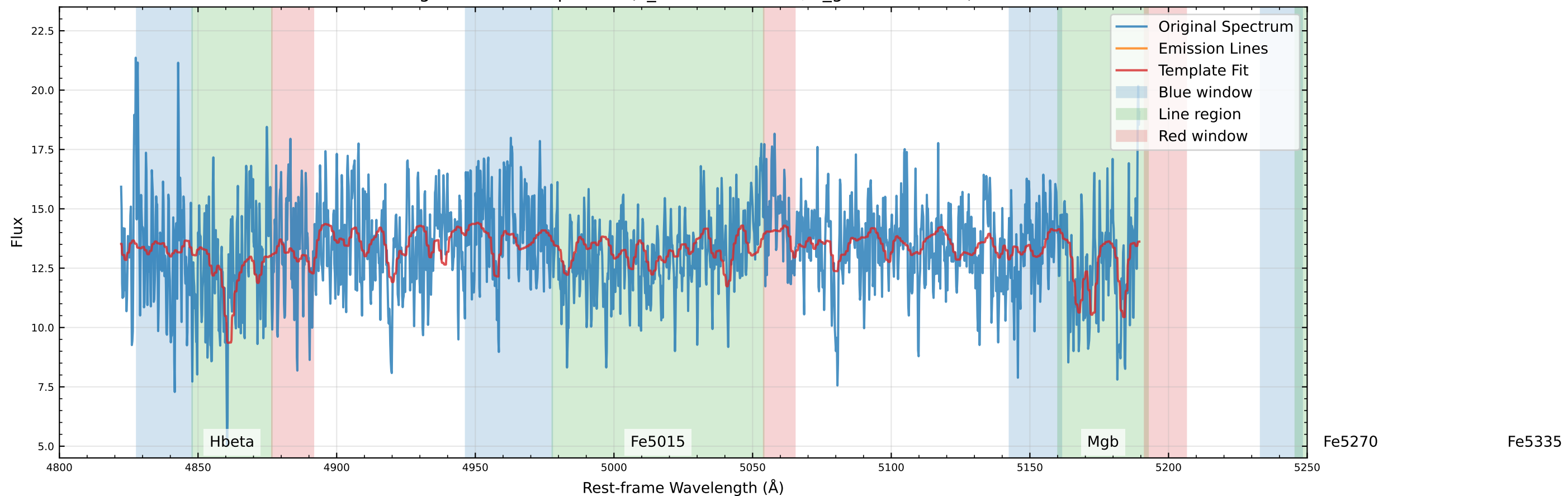
Original Data Comparison (v_star=-49.5 km/s, v_gas=25.8 km/s)
