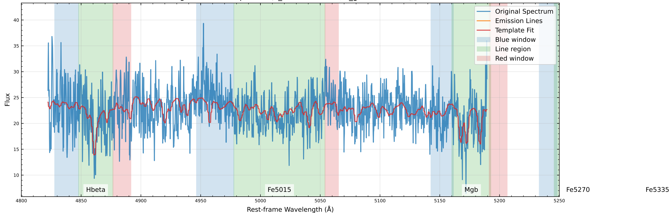
Original Data Comparison (v_star=-5.4 km/s, v_gas=-8.1 km/s)
