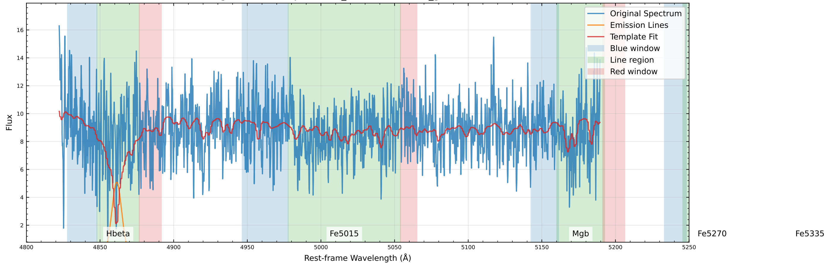
Original Data Comparison (v_star=-0.6 km/s, v_gas=43.9 km/s)
