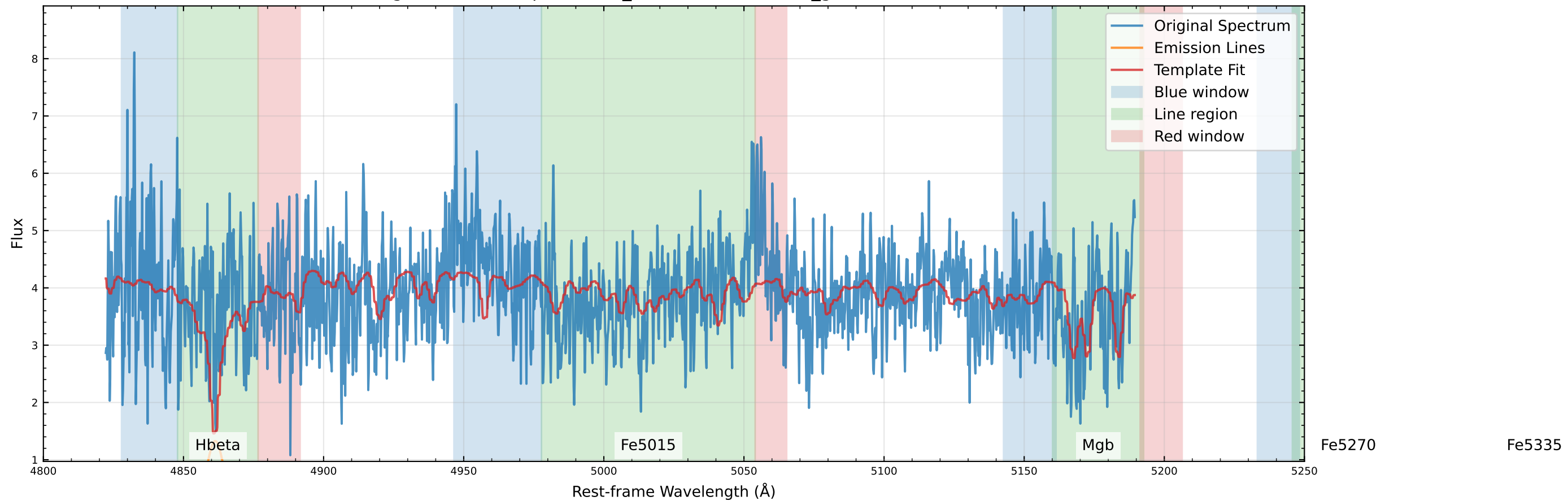
Original Data Comparison (v_star=-109.2 km/s, v_gas=-105.5 km/s)
