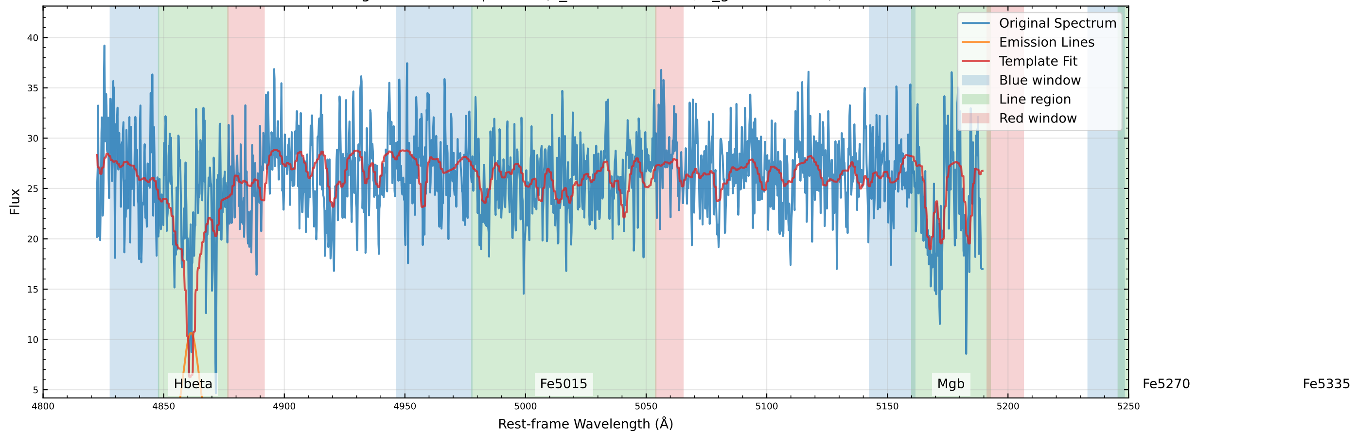
Original Data Comparison (v_star=-53.2 km/s, v_gas=7.3 km/s)
