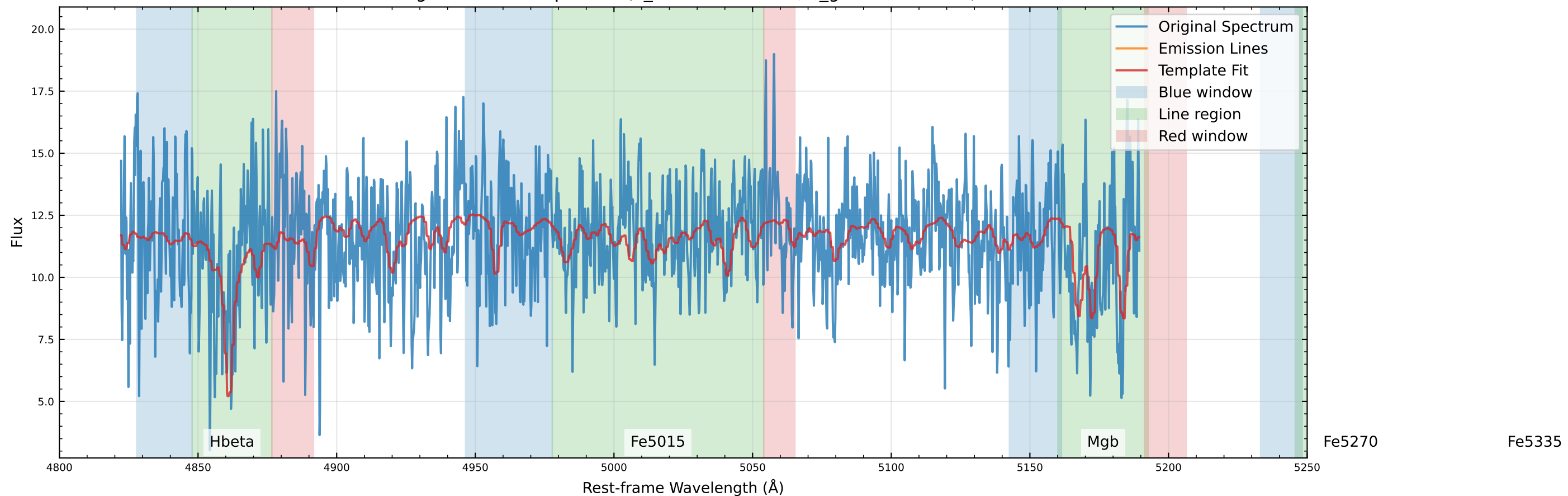
Original Data Comparison (v_star=-41.7 km/s, v_gas=-91.5 km/s)
