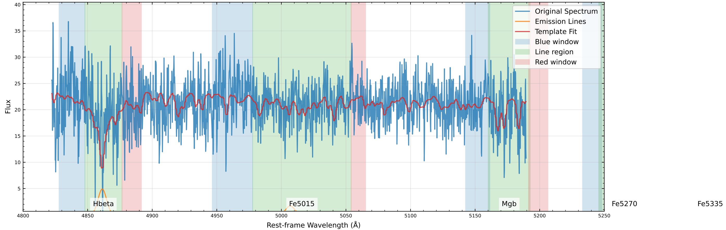
Original Data Comparison (v_star=25.1 km/s, v_gas=117.1 km/s)
