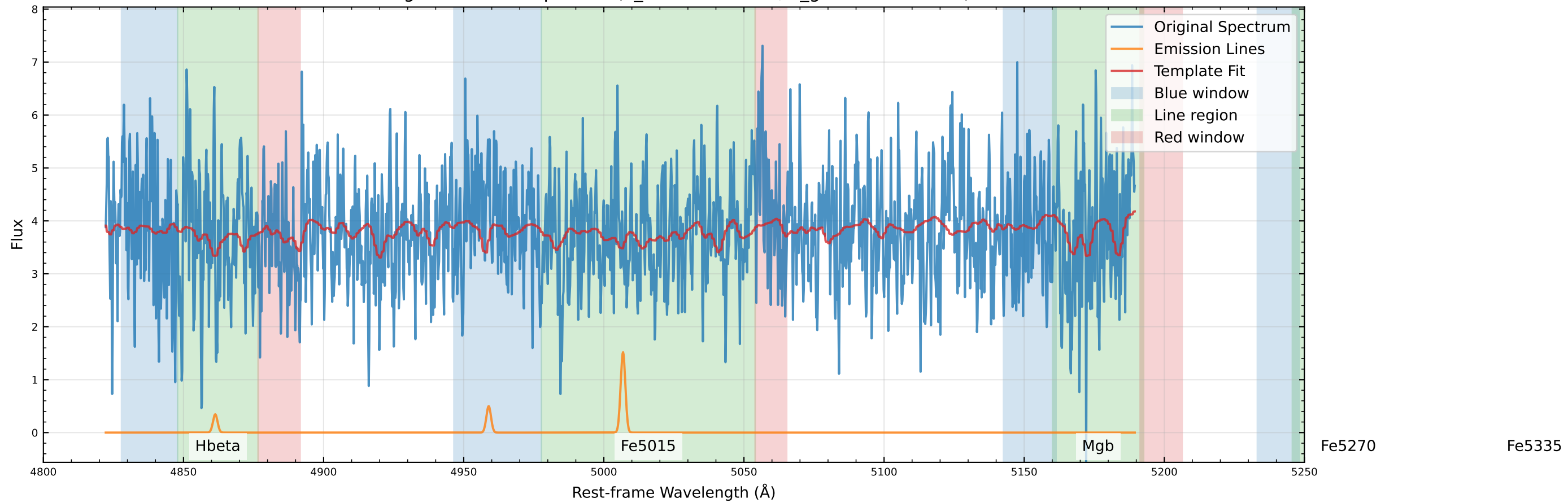
Original Data Comparison (v_star=-0.9 km/s, v_gas=-127.3 km/s)
