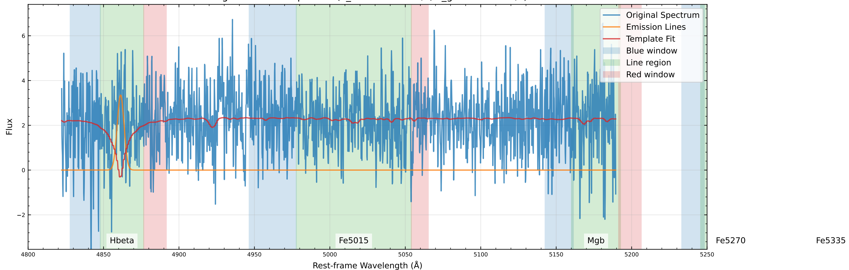
Original Data Comparison (v_star=-35.6 km/s, v_gas=-84.3 km/s)
