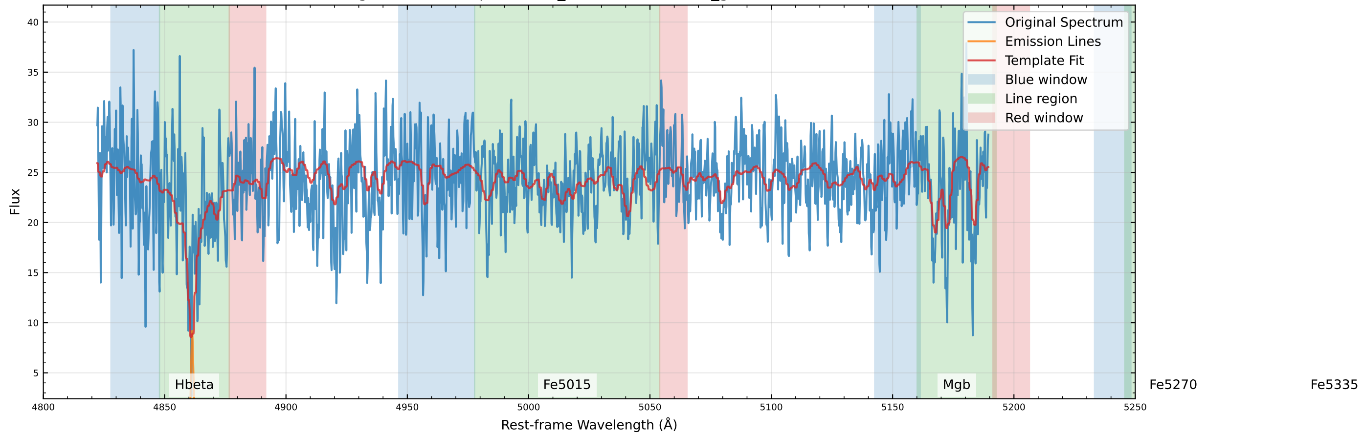
Original Data Comparison (v_star=-10.7 km/s, v_gas=31.5 km/s)
