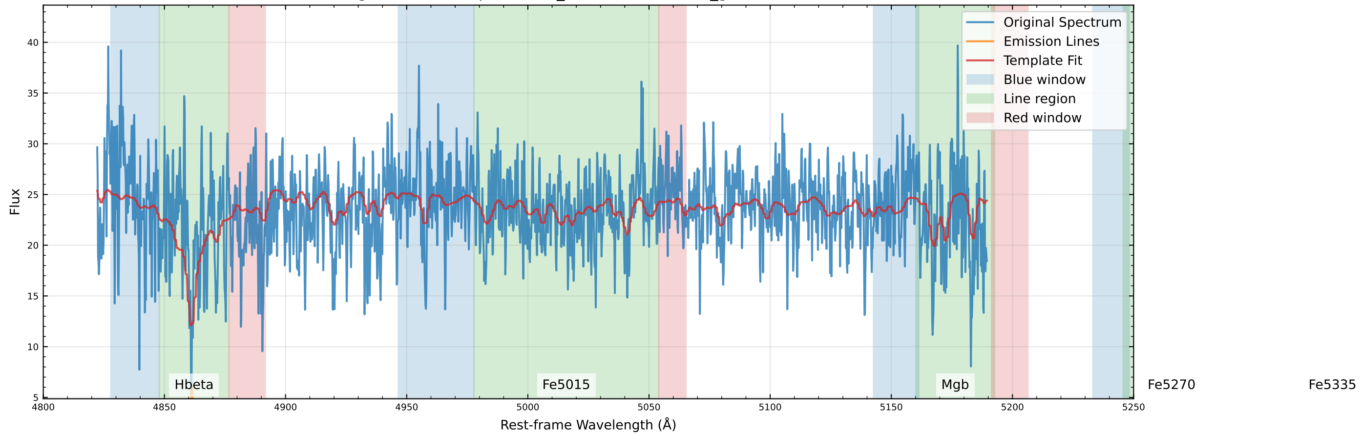
Original Data Comparison (v_star=-12.2 km/s, v_gas=86.5 km/s)
