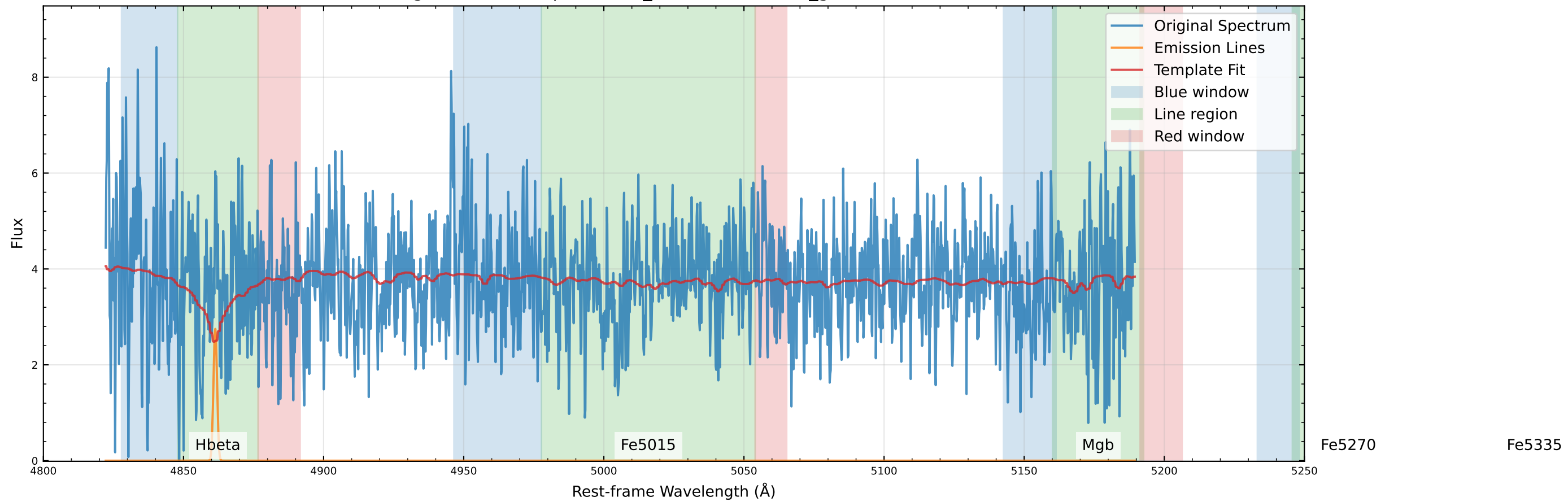
Original Data Comparison (v_star=-8.1 km/s, v_gas=16.0 km/s)
