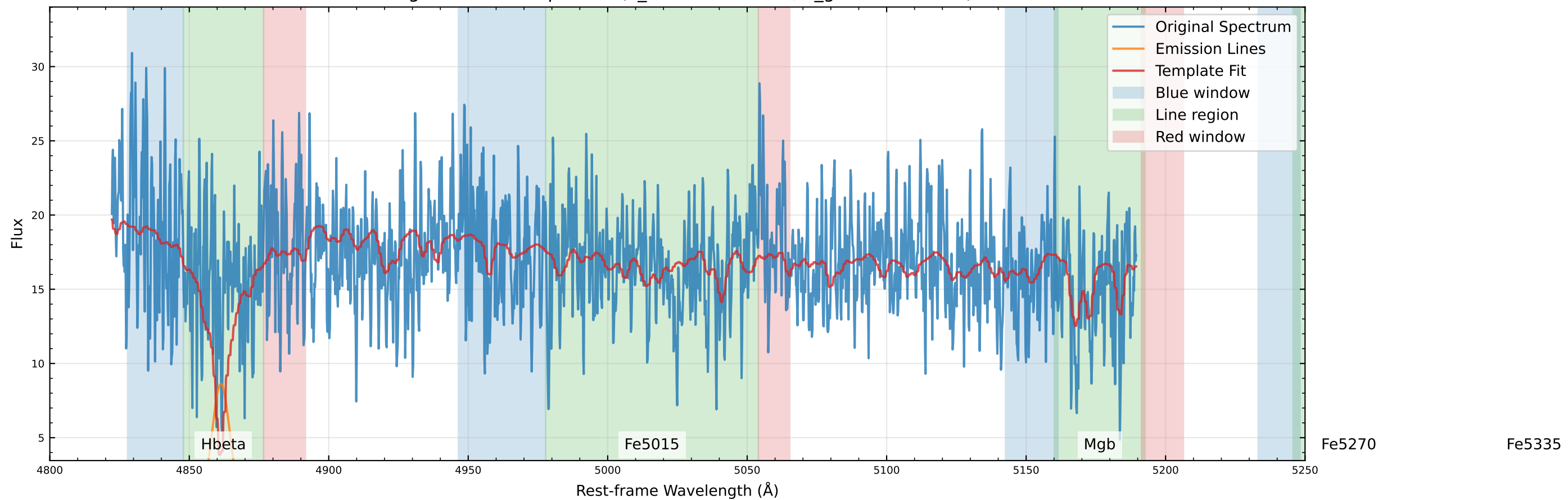
Original Data Comparison (v_star=-13.3 km/s, v_gas=-18.3 km/s)
