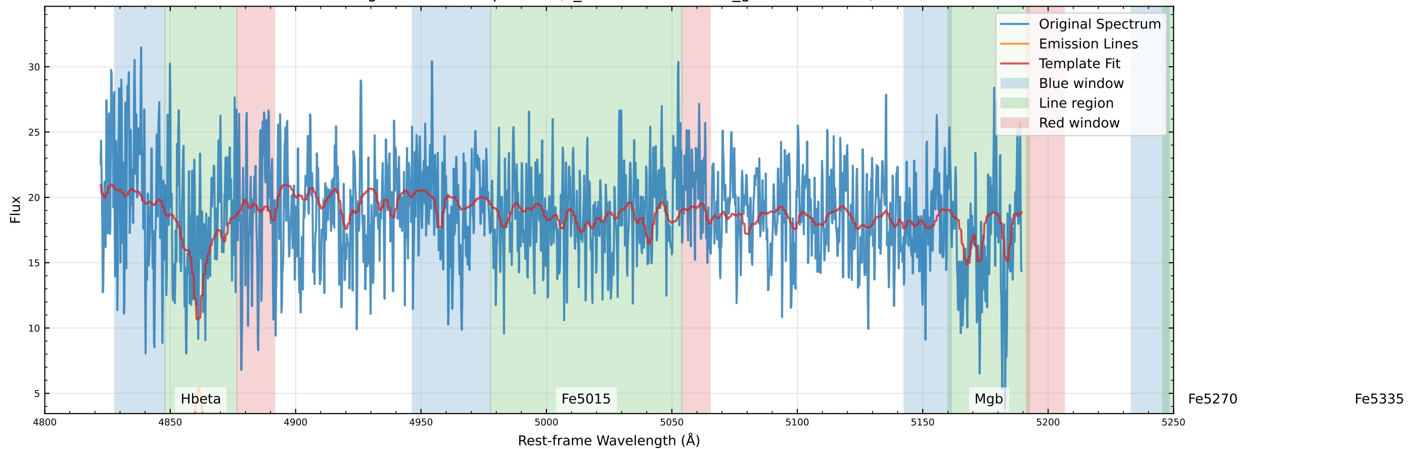
Original Data Comparison (v_star=-35.2 km/s, v_gas=-45.5 km/s)
